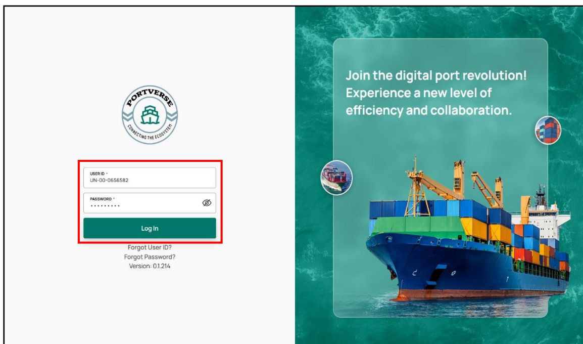
Figure 4 - Login Screen
